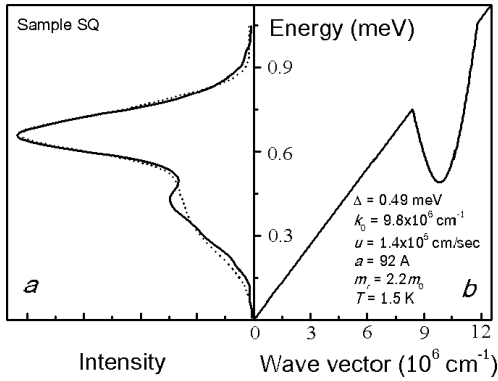
Fig. 3. Experimental PL spectrum of a biexcitonic liquid in a \beta -ZnP 2 crystal (solid curve) and its approximation by the theoretical spectrum (dashed curve) (a); the dispersion curve for the elementary excitations of the quantum biexcitonic liquid with the parameters obtained by fitting the theoretical PL spectrum to the experimental spectrum (b). Excitation intensity is 3 kW/cm 2 .
