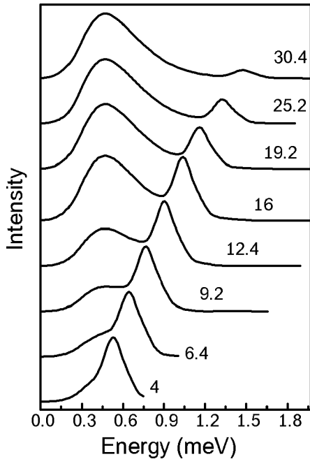
Fig. 2. Evolution of the theoretical PL spectrum of a quantum biexcitonic liquid under variation of the square of the excitation intensity (density of the liquid): n \propto I_{\text{exc}}^2 . The curves are labeled with the value of I_{\text{exc}}^2 in arbitrary units.
