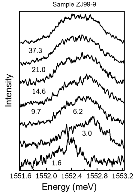
Fig. 5. Evolution of the experimental PL spectrum of a biexcitonic liquid in a \beta -ZnP 2 crystal under variation of the square of the excitation intensity. The curves are labeled by the value of I_{exc}^2 in (kW/cm 2 ) 2 .
