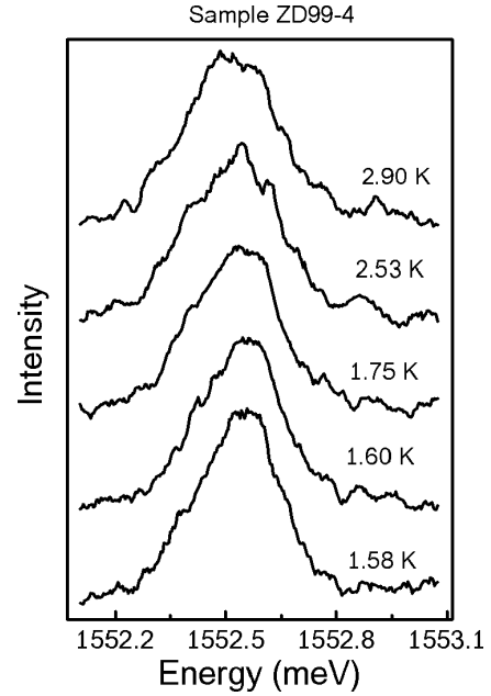
Fig. 4. Evolution of the experimental PL spectrum of a biexcitonic liquid in a \beta -ZnP 2 crystal under variation of temperature of the sample at the point of excitation. Excitation intensity is 4.8 kW/cm 2 .
