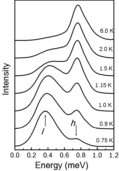
Fig. 1. Evolution with temperature of the calculated photoluminescence spectrum of a quantum biexcitonic liquid with a phonon-roton dispersion relation for the elementary excitations. The arrow labeled l indicates the low-energy ( l ) component of the spectrum, and the arrow h the high-energy ( h ) component.
