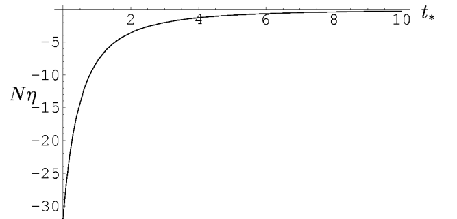
Fig. 1. Plot of N\eta , where \eta is given by Eq. (19), as a function of t_* > 0 .
