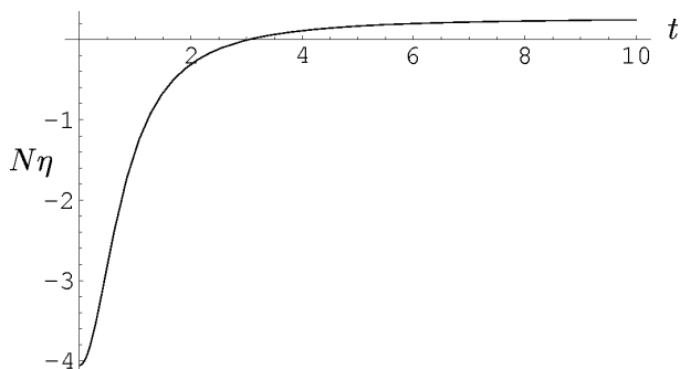
Fig. 6. Plot of N\eta , where \eta is given by Eq. (31), as a function of t .
