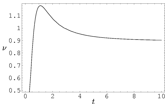
Fig. 7. Plot of \nu , where \nu is given by Eq. (32) with N = 10 , as a function of t .
