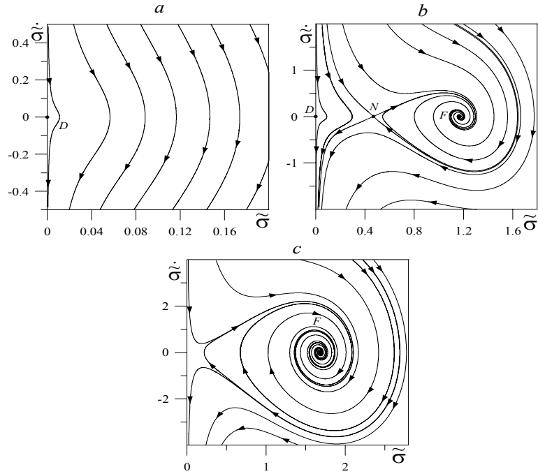
Fig. 2. The phase portraits corresponding to the parameters of Fig. 1: a – DF mode corresponds to the curve 1 in Fig. 1; b – SS – curve 2 in Fig. 1; c – SF – curve 3 in Fig. 1
