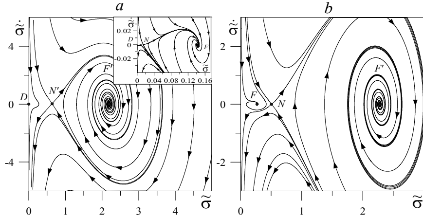
Fig. 4. The phase portraits corresponding to the parameters of Fig. 3: a – SS+SF mode corresponds to the curve 3 in Fig. 3; b – MSF+SF – curve 4 in Fig. 3
