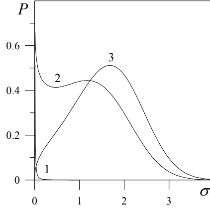
Fig. 1. The distribution function of shear stress for the second-order transition at g = 0, 2 , \tau_\sigma = \tau_\varepsilon = 0, 1 , \tau_\lambda = 0, 2 , and I = 5 . The curves 1, 2, 3 correspond to the temperatures T_e = 5, 16, 20 , respectively
