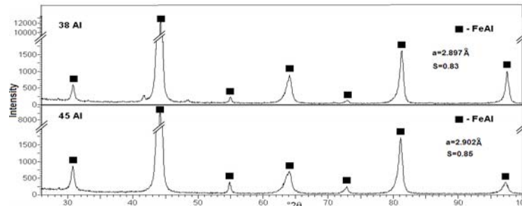
Fig. 1. X-ray diffraction patterns of \text{Fe}_{62}\text{Al}_{38} and \text{Fe}_{55}\text{Al}_{45} samples annealed at 1000^\circ\text{C} for 48 hours
