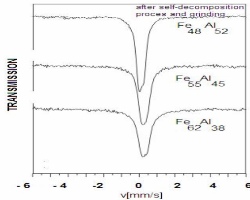
Fig. 2. The ^{57}\text{Fe} Mössbauer transmission spectra for \text{Fe}_{62}\text{Al}_{38} (a), \text{Fe}_{55}\text{Al}_{45} (b) alloys annealed for 48 h at 1000^\circ\text{C} and \text{Fe}_{48}\text{Al}_{52} obtained by self-decomposition method and intensive grinding
