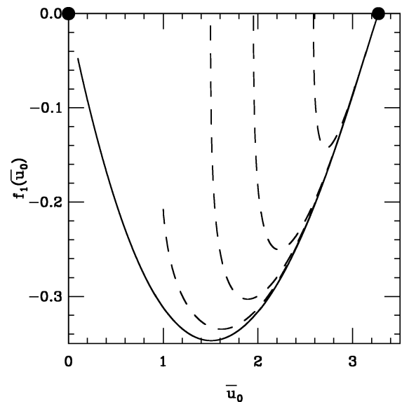
Fig. 4. Graphical representation of the Wilson differential flows (dashed curves), in \mathcal{S}_c at d = 3 , projected on the u_0 -axis — i.e. f_1(\bar{u}_0) = -d\bar{u}_0(l)/dl . In the infra-red direction, any (dashed) curve exponentially approaches a limiting (full) curve which coincides with the differential-momentum-scale-dependence carried by the ultimate Wilson flow emerging from the Gaussian fixed point P_G (left-hand full circle). The function f_1(\bar{u}_0) is numerically determined along this flow corresponding to the trajectory T_1 in \mathcal{S}_c . Notice that the convergence is numerically well controlled independently of whether the initial point is chosen close to P_G or not. The righthand full circle indicates the infra-red stable fixed-point-value u_0^* = 3.27039 \dots .
