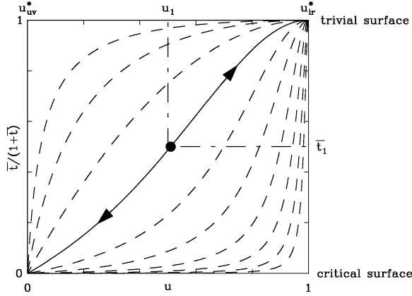
Fig. 1. Qualitative representation of the momentum–scale dependence for the \phi_d^4 field theory with d < 4 . The curves drawn (see also fig. 2) are obtained from assuming \nu = 1/2 and a \beta -function of the form \beta(x) = x(x - 1) ; \tilde{t}(\lambda) stands for \tilde{t}(\lambda)/\lambda^2 . Among the continuous family of curves (dashed curves) a measurement is required in order to choose (full circle) one curve (full curve). An upward arrow indicates the infra-red direction, a downward arrow the ultra-violet direction. See text for more detail.
