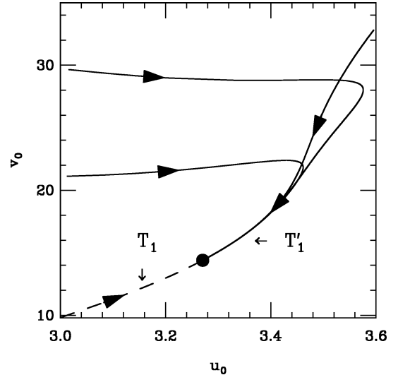
Fig. 6. The "unusual" infra-red stable one-dimensional submanifold in \mathcal{S}_c ( T'_1 ) obtained from Eq. (3.11) with d = 3 (projection onto the plane (u_0, v_0) ). The full circle represents the infra-red stable fixed point f^* and the usual "renormalized trajectory" T_1 emerging from P_G is partially drawn (dashed curve). Arrows indicate the infra-red direction.
