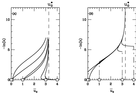
Fig. 5. Functional momentum-scale dependence displayed by \bar{u}_0(l) (projection onto the u_0 -axis of \mathcal{S} ) along definite Wilson’s flows on \mathcal{S}_c (A). Open circles indicate the initial points chosen in \mathcal{S}_c . Each full curve in (A) provides a determination of the functional momentum-scale dependence. In order to emphasize where the effective field theory (see section IIID2) practically occurs in each case, on figure (B) we have artificially translated the “time” scales l = -\ln(\lambda) (vertical dashed lines) such that each actual Wilson’s flow of (A) “hits” a given unique value of \bar{u}_0 at the same “time”. The unique functional flow so obtained illustrates the underlying unique differential flow of fig. 4.
