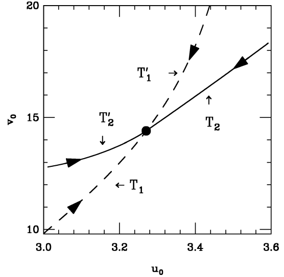
Fig. 8. The two infra-red attractive submanifolds in \mathcal{S}_c^{(2)} T_2 and T'_2 (full curves) of same degree of stability but lower than on T_1 and on T'_1 (dashed curves) (projection onto the plane (u_0, v_0) ). The initial values chosen are r_{0c}(0) = -0.5832891\dots , u_0(0) = 6.6615188\dots , v_0(0) = 0 ( T_2 ) and r_{0c}(0) = -0.42788517\dots , u_0(0) = 2 , v_0(0) = 26.13624 ( T'_2 ).
