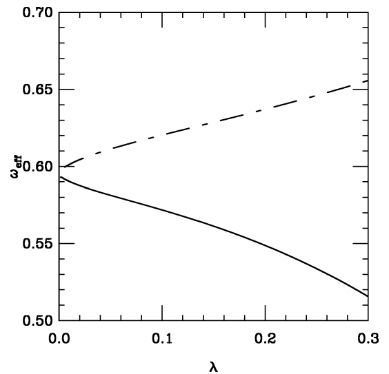
Fig. 7. Effective correction-exponent \omega_{\text{eff}}(l) (Eq. (3.23) with l = -\ln \lambda ) along T_1 (full curve) and along T'_1 (dot-dashed curve). The estimate of the value of \omega is 0.5955 \pm 0.0025 .
