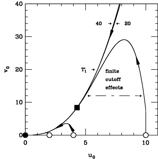
Fig. 9. Wilson's flows on the critical surface \mathcal{S}_c obtained from integration of Eq. (3.11) at d = 4 (projection onto the plane (u_0, v_0) ). Open circles indicate the initial points chosen on the canonical surface of \mathcal{S}_c : (u_0(0), r_{0c}(0)) = (2, -0.035806374\dots) ; (4, -0.068682647\dots) ; (10, -0.1577796\dots) . Two flows initialized at (20, -0.2892822265\dots) and (40, -0.52207031\dots) are partially reproduced. The full circle represents the infra-red stable fixed point P_G . Arrows indicate the infra-red direction. The square roughly indicates where the effective field theory could make sense for the Wilson trajectory initialized at u_0(0) = 10 .
