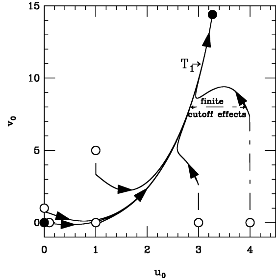
Fig. 3. Projection onto the plane (u_0, v_0) of some Wilson’s trajectories on the critical surface \mathcal{S}_c (after integration of Eq. (3.11) at d = 3 ). Full circles indicate the locations of the Gaussian ( P_G ) and the non-trivial ( f^* ) fixed points respectively. Arrows indicate the infra-red direction. Open circles indicate the locations of the initial points. The values of the initial sets of coordinates (r_{0c}(0), u_0(0), v_0(0)) are the following: (-0.014175577 \dots, 0.1, 0) , (-0.116887403 \dots, 1, 0) , (-0.299586913 \dots, 3, 0) , (-0.381259493 \dots, 4, 0) , (-0.180075418 \dots, 1, 5) , (-0.025823782 \dots, 0, 1) the other coordinates being set equal to zero. The full curves represent Wilson’s trajectories entirely plunged in \mathcal{S} . The “vertical pieces” (dot-dashed lines) are numerically undetermined parts of the projected Wilson trajectories. They reflect the lack of accuracy in our determination of v_0(l) for small l .
