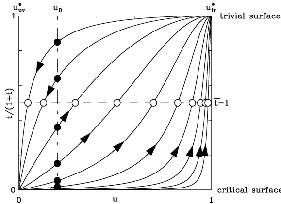
Fig. 2. Use of the \phi_d^4 field theory in the study of critical phenomena. The presentation is similar to fig. 1. See text for a discussion of the figure.
