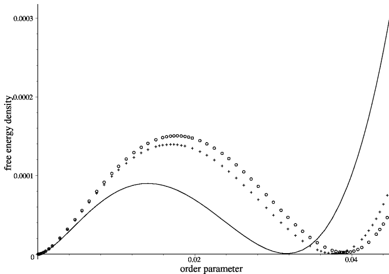
Fig. 2. The function f(\varphi) for Al films of thickness L_0 = 0.1 \mu\text{m} : the solid line (—) corresponds to ET, the line of crosses (+) represents LT, and the line of circles (o) stands for SLT. All curves are calculated for T_{\text{eq}} corresponding to the respective variant of the theory (see the text).
