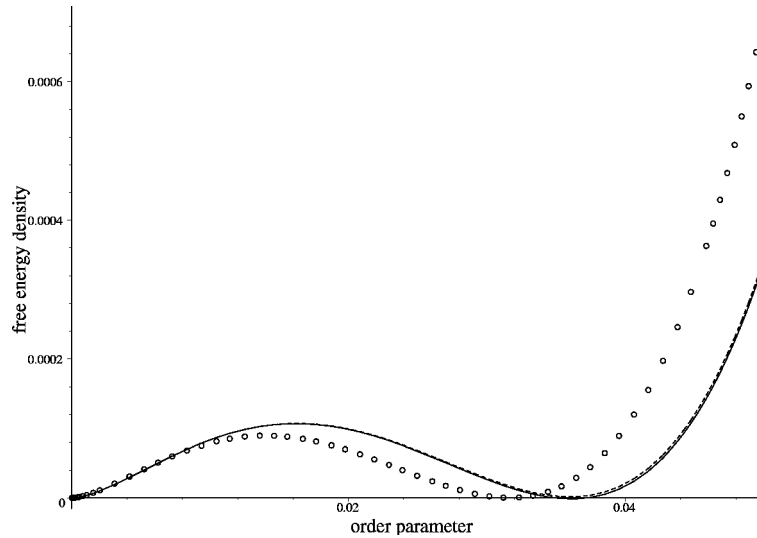
Fig. 3. The function f(\varphi) calculated from the ET for Al films of thickness L_0 = 0.1 \mu\text{m} and different cutoffs \Lambda : the solid line (—) corresponds to \Lambda = \pi/\lambda_0 , the dashed line represents the case \Lambda = 1/\lambda_0 , and the line of circles (o) stands for \Lambda = \pi/\xi_0 . All curves are calculated at the respective T_{\text{eq}} (see the text).
