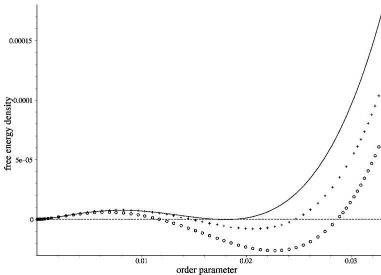
Fig. 1. The function f(\varphi) for Al films of thickness L_0 = 0.4 \mu\text{m} : the solid line corresponds to ET, the line of crosses (+) represents LT, and the line of circles (o) stands for SLT. All curves are calculated for T_{\text{eq}} corresponding to ET (see the text).
