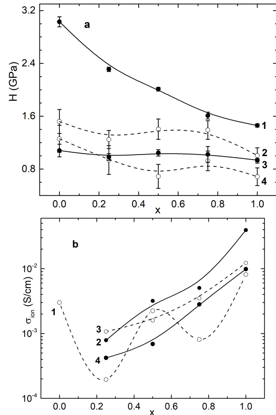
Fig. 2. The compositional dependences of microhardness at P = 0.5 \text{ N} (a) and ionic component of electrical conductivity (b) for (\text{Cu}_{1-x}\text{Ag}_x)_7\text{SiS}_5\text{I} crystals (1) and ceramics with different grain size: 12 \mu\text{m} (2), 5 \mu\text{m} (3), 3 \mu\text{m} (4).
