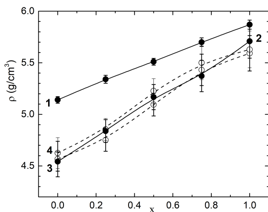
Fig. 3. The compositional dependences of density for (\text{Cu}_{1-x}\text{Ag}_x)_7\text{SiS}_5\text{I} crystals (1) and ceramics with different grain size: 12\ \mu\text{m} (2), 5\ \mu\text{m} (3), 3\ \mu\text{m} (4).
